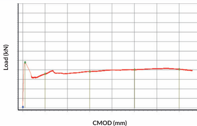
Flexural tensile strength of Fiber-Reinforced Concrete EN 14651
