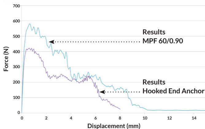
MPF 60/0.90 vs. Hooked End Anchorage Pull-out test in ABAQUS \Rightarrow Force displacement
